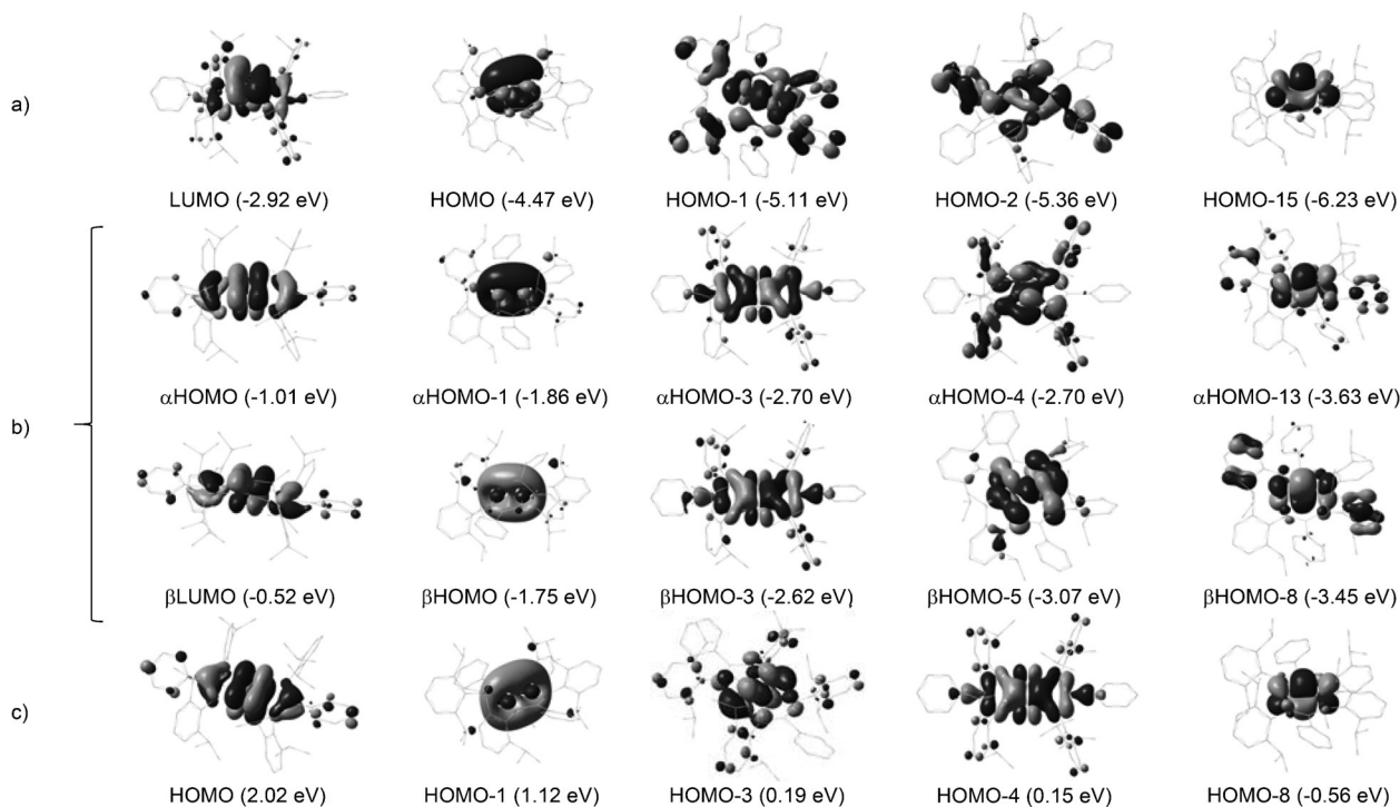
Figure 3. The frontier molecular orbitals signifying \delta , \pi , and \sigma bonding of a) [\text{Mo}_2(\mu\text{-}\kappa^2\text{-PhB}(\text{N-2,6-}^i\text{Pr}_2\text{C}_6\text{H}_3)_2)_2] ( 5 ), b) [\text{Mo}_2(\mu\text{-}\kappa^2\text{-PhB}(\text{N-2,6-}^i\text{Pr}_2\text{C}_6\text{H}_3)_2)_2]^- ( 6 ), and c) [\text{Mo}_2(\mu\text{-}\kappa^2\text{-PhB}(\text{N-2,6-}^i\text{Pr}_2\text{C}_6\text{H}_3)_2)_2]^{2-} ( 7 ).
